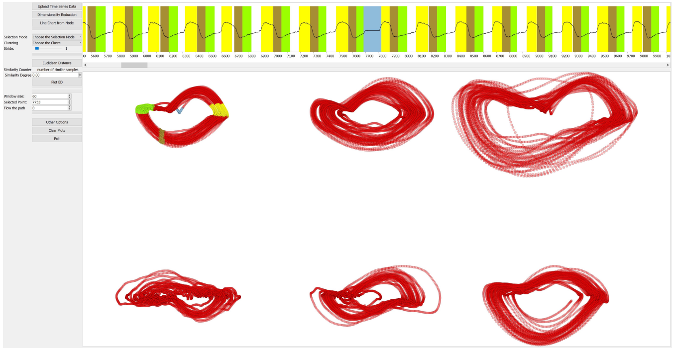
Fig. 5. The main user interface of our system on data from a deployment on pulmonary fibrosis data. Top: zoomed time-series chart with overlaid colored regions corresponding to the chosen clusters in the scatter plot. The user can zoom in both charts to see more detail. The left side of the interface shows some buttons and parameters which can be modified based on the user desires. Each cluster, outlier, and transition can be colored with a different color to be identified and compared.
