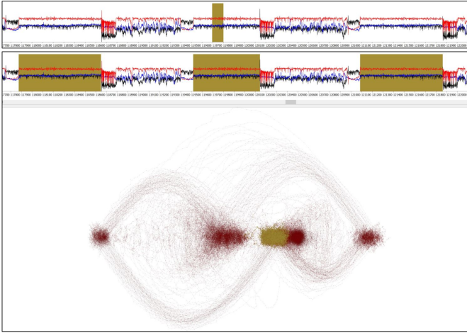
Fig. 4. Selection using similarity. The user selects part of the data from the time-series view (top). All other data that matches below a threshold based on Euclidean distance are labelled the same. In this case the selection corresponds to the “Surface swimming” cluster.
