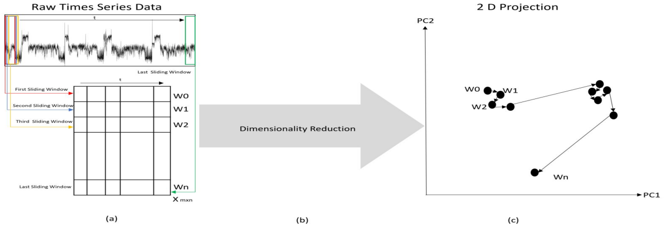
Fig. 3. Our system approach which consists of three major steps. (a) preprocessing, (b) dimensionality reductions, and (c) visual exploration.
